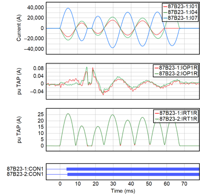
Fig. 6. 87B23-1 and 87B23-2 event data.
